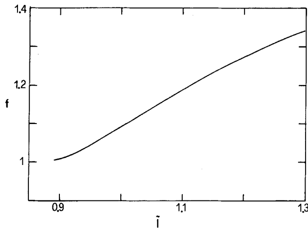
FIGURE 1 The universal function f(\tilde{I}) . The function extends to the region \tilde{I} < 1 because of the hysteresis of the rotational motion.
